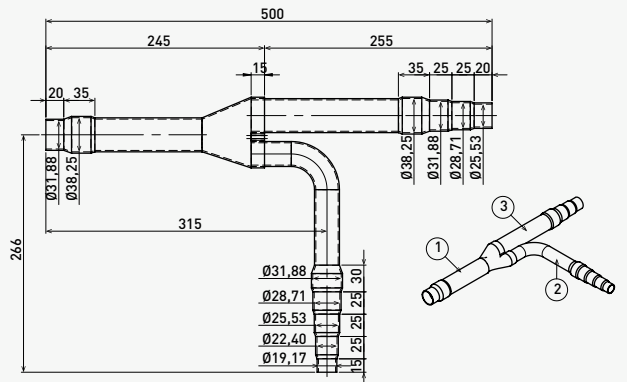
Gas piping
