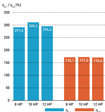
MF4 Series seasonal efficiency.
