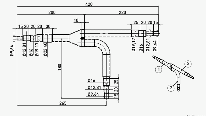
Liquid piping
