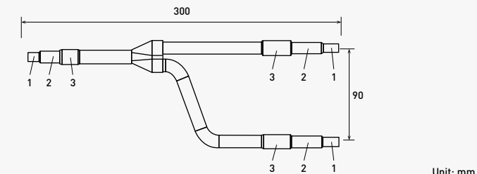
Liquid piping
