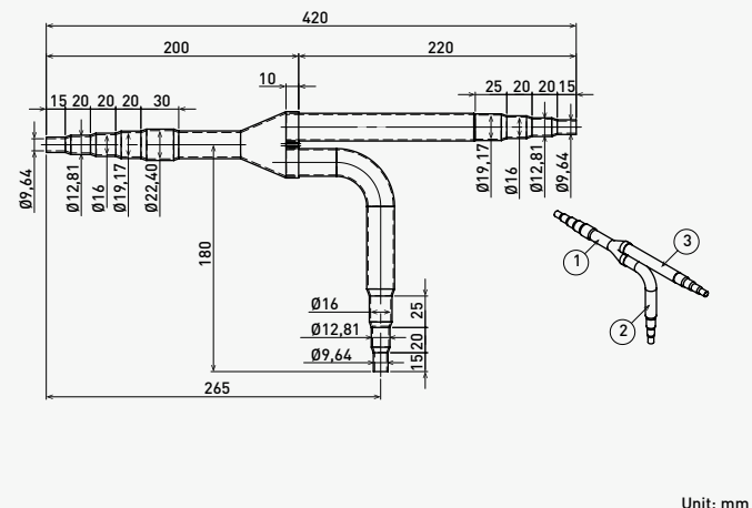
Liquid piping
