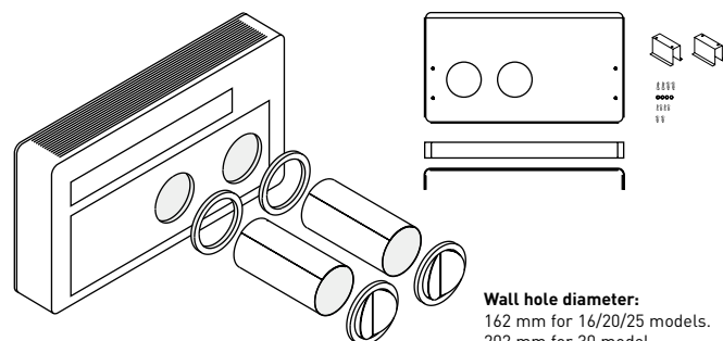
*The outside grille varies by version. Shown: P-MOZ16/20/25/30IC5-E.
