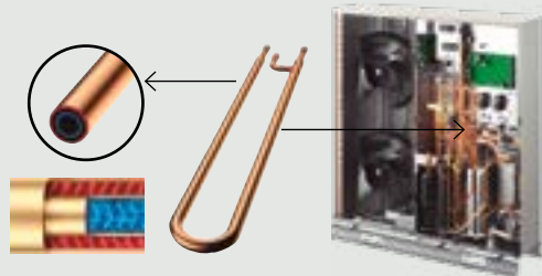
Image of the Aquarea T-CAP J Series Mono-bloc.
