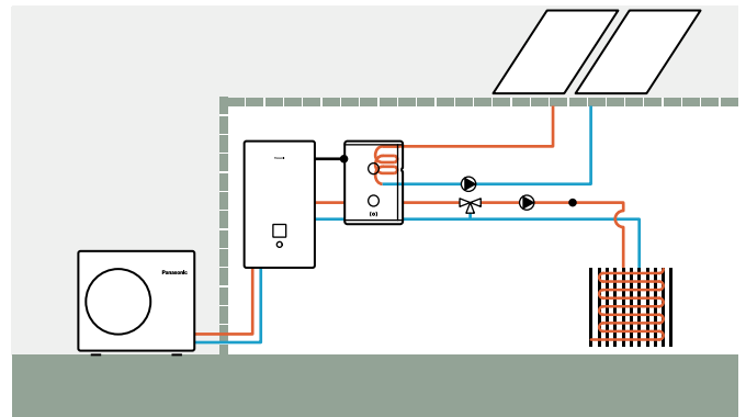
Aquarea Split Bi-bloc: Buffer tank with solar and mixing valve
