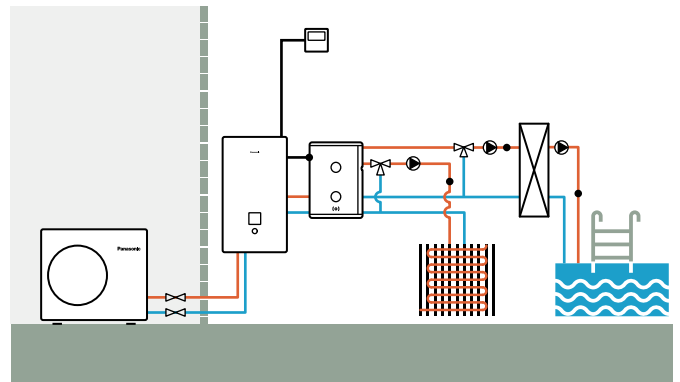
Aquarea Hydraulic Bi-bloc: 2 zones with external kit, buffer tank and swimming pool
